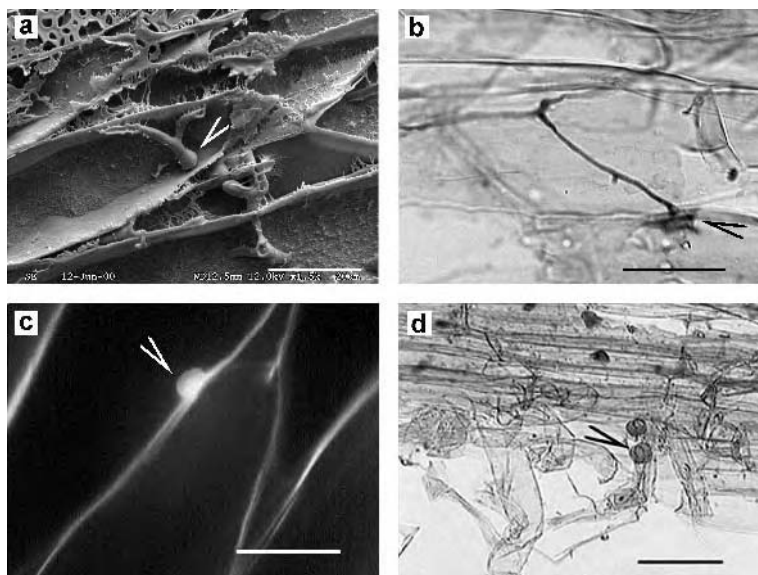
Fig. 11.2. a Formation of appressoria (arrow) by Arthrobotrys oligospora during penetration of the epidermis of barley roots. (From Bordallo et al. 2002, courtesy of Blackwell Science). b Colonisation of tomato roots by Pochonia chlamydosporia . Note appressorium and cell wall protein apposition (arrow). (From Bordallo et al. 2002, courtesy of Blackwell Science). c Colonisation of barley roots by A. oligospora . Callose deposit in papillae (arrow) stained with Sirofluor. (From Bordallo et al. 2002, courtesy of Blackwell Science). d Colonisation of tomato roots by Pochonia chlamydosporia . Note externally produced chlamydospores (arrow). (From Bordallo et al. 2002, courtesy of Blackwell Science). Bars a , c 20 \mu\text{m} ; b , d 30 \mu\text{m}
