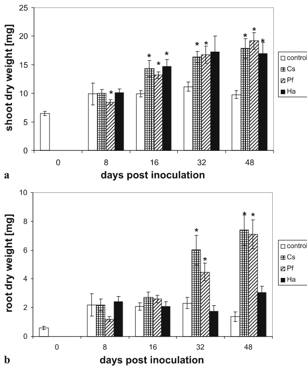
Fig. 15.1. Influence of colonisation on dry weights of shoots (a) and roots (b) of Larix decidua , cultivated for 3 months axenically in a synthetic medium in expanded clay and inoculated at day 0 with either an endophyte, Cryptosporiopsis sp. (Cs) or Phialocephala fortinii (Pf), or a pathogen, Heterobasidion annosum (Ha). n = 29-55 , *P < 0.05 , significant in comparison to the control according to Kruskal-Wallis ANOVA on ranks (Schulz et al. 2002)
