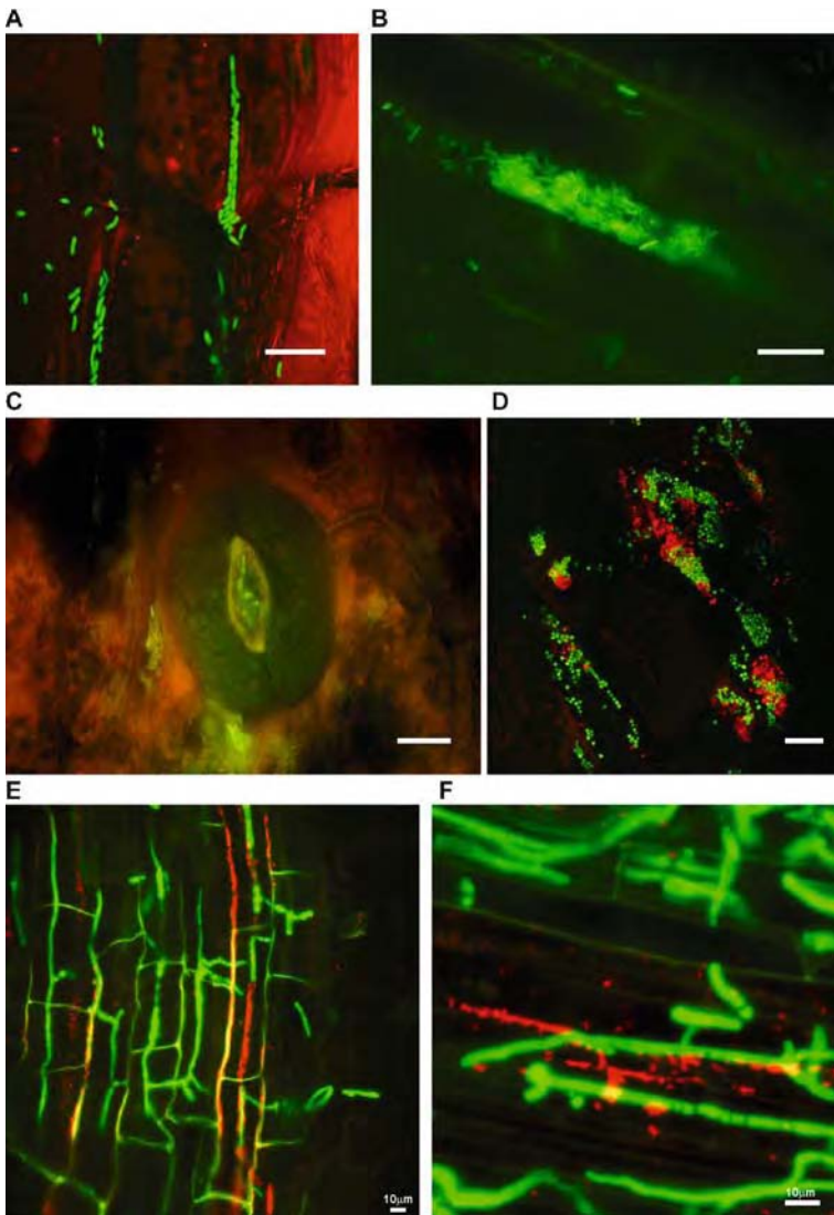
Fig. 18.3. A–F Confocal laser scanning microscopy (CLSM) analysis of tomato surfaces colonised by Pseudomonas spp. and Fusarium oxysporum f. sp. radicum lycopersici labelled with autofluorescent proteins. Tomato seedlings were grown upon inoculation in a gnotobiotic sand system. Plants were taken out after 7 days of growth and examined for the presence of green fluorescent protein ( gfp )- or red fluorescent protein ( rfp )-expressing organisms. A Colonisation of the root surface by P. fluorescens expressing enhanced GFP ( egfp ). B Colonisation of the lumen of a root cell. C Colonisation of a stoma. D Simultaneous imaging of root surface colonisation by a mixture of P. putida PCL1444 expressing egfp and P. putida PCL1446 expressing rfp . E , F Interactions between P. chlororaphis PCL1391 expressing rfp and the phytopathogenic fungus Fusarium oxysporum f. sp. radicum lycopersici expressing gfp during colonisation. Bars 10 µm. D courtesy of E. Lagendijk; E , F courtesy of T. Lagopodi and A. Bolwerk
