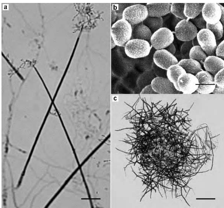
Fig. 13.1. a–c Morphology of Oidiiodendron maius in axenic culture. a Tall, erect, melanized conidiophores and small, hyaline arthroconidia of O. maius (UAMH 9749) viewed under light microscopy. b Chains of arthroconidia of O. maius (UAMH 8920), showing asperulate ornamentation visible under scanning electron microscopy. c Sterile peridial elements produced by O. maius (UAMH 9749) on thalli of Cladonia mitis . The cage-like peridial elements resemble the cleistothecia of species of Myxotrichum . Bars a 40 \mu m, b 5 \mu m, c 80 \mu m
