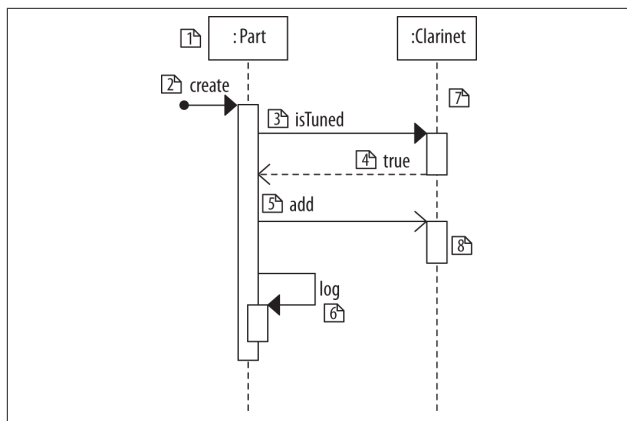
Figure C-7. Sequence diagrams
